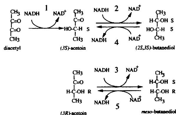
Figure 3. Reactions catalysed by the diacetyl (acetoin) reductase from B. stearothermophilus .
